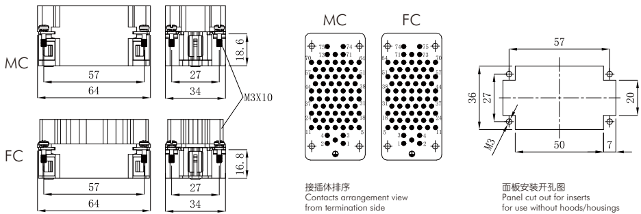
Dimensions mm
