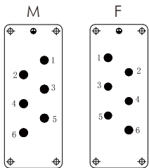
接插体排序 Contacts arrangement view from termination side
