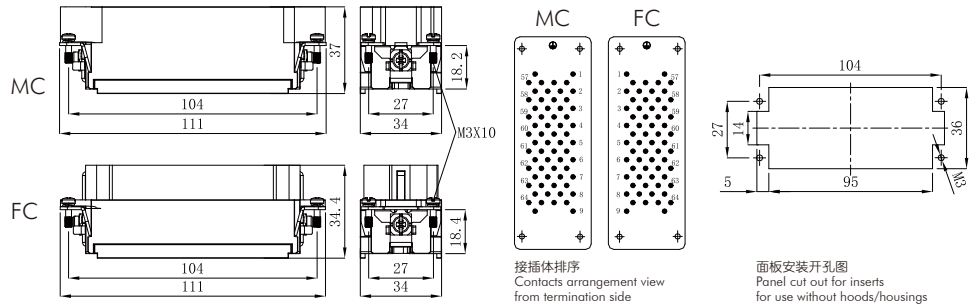
Dimensions mm
