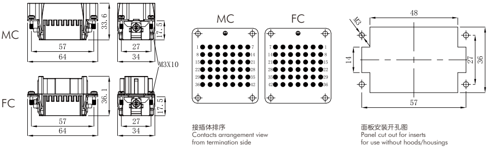
Dimensions mm
