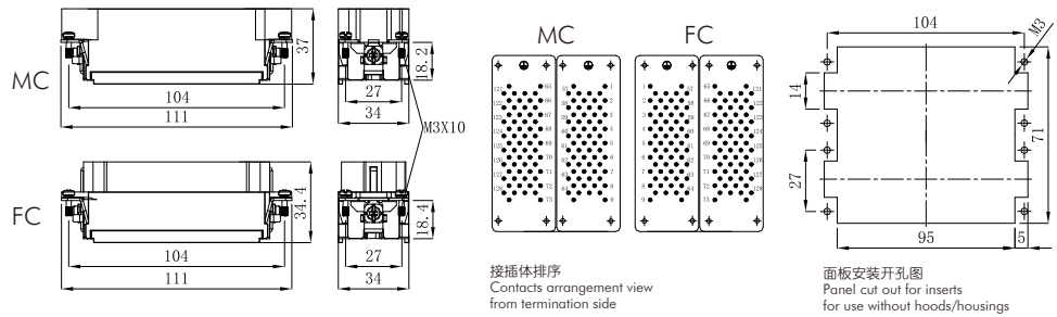
Dimensions mm
