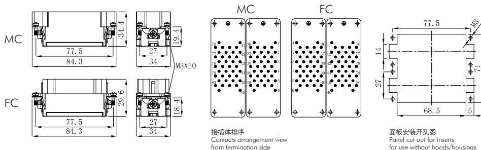
Dimensions mm
