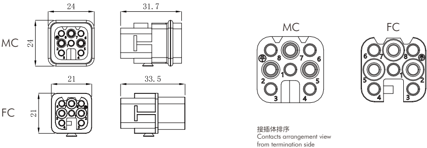
Dimensions mm
