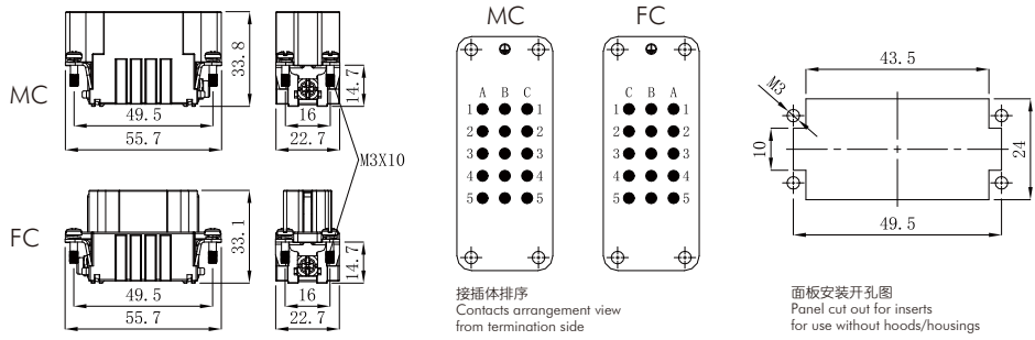
Dimensions mm
