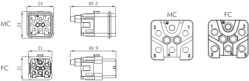
Dimensions mm
